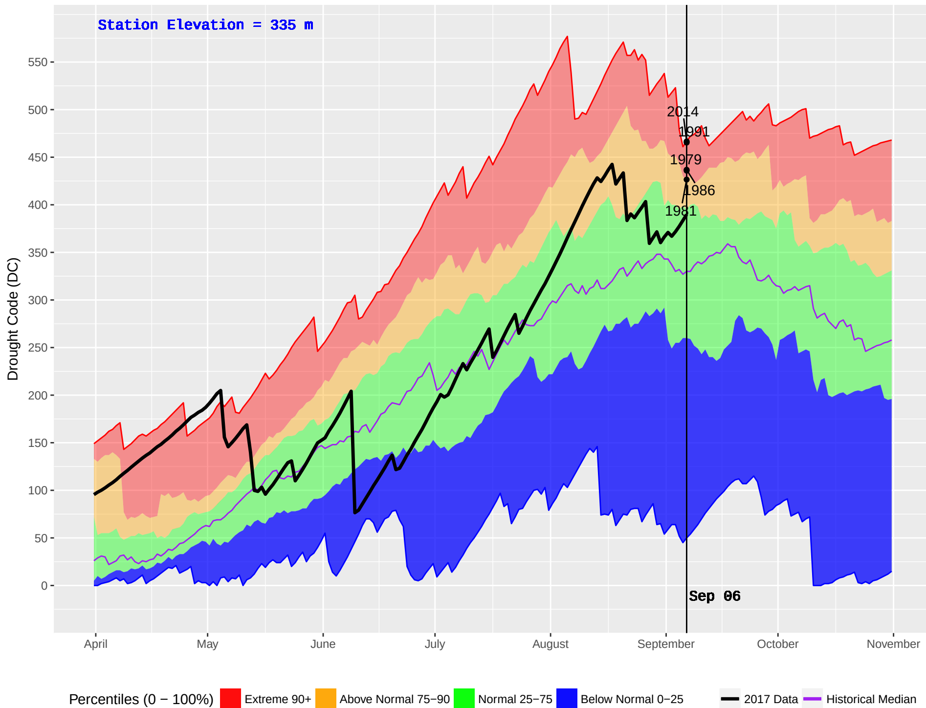
KISPIOX HUB (428) : Historical (1970–2016) and Current (2017) Noon Drought Code (DC)
